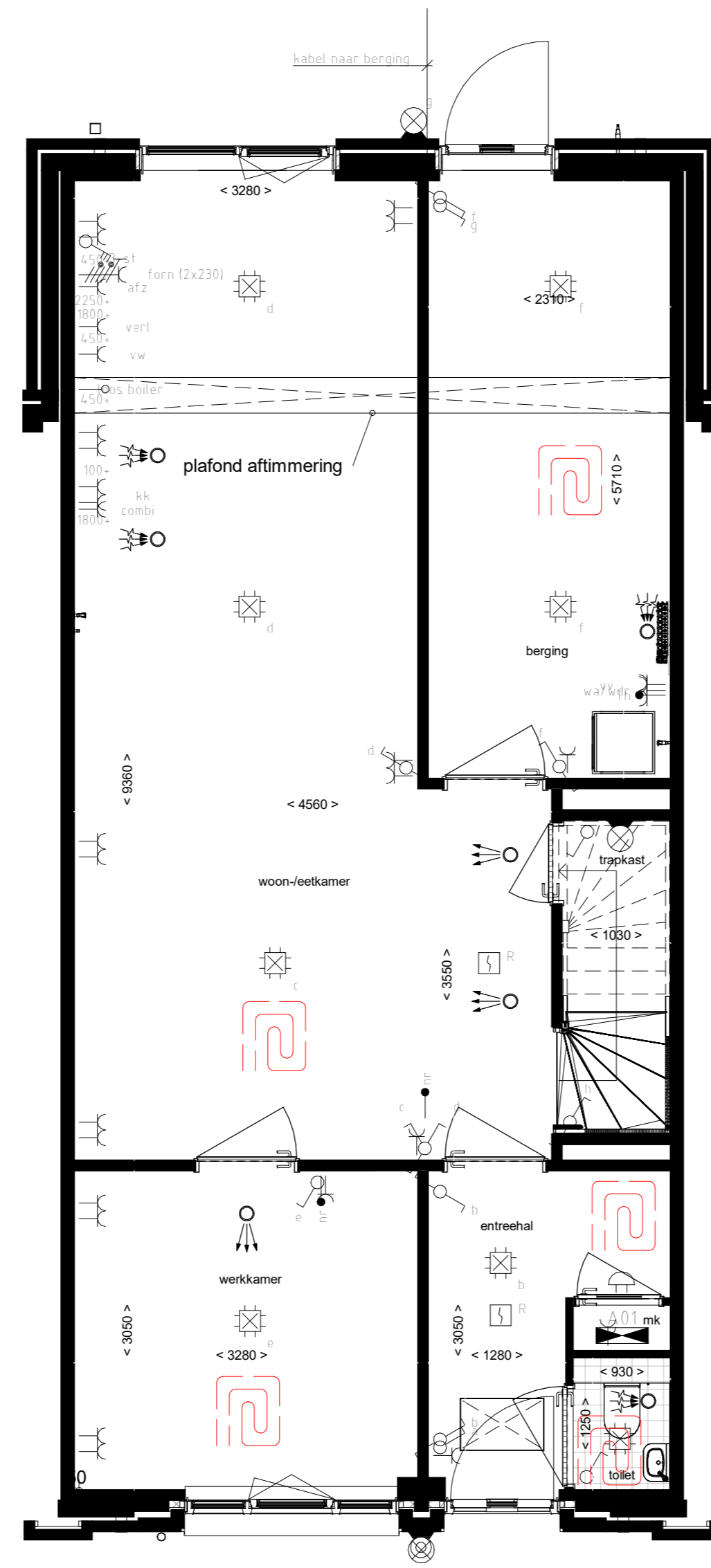
Begane grond - indeling variant A
